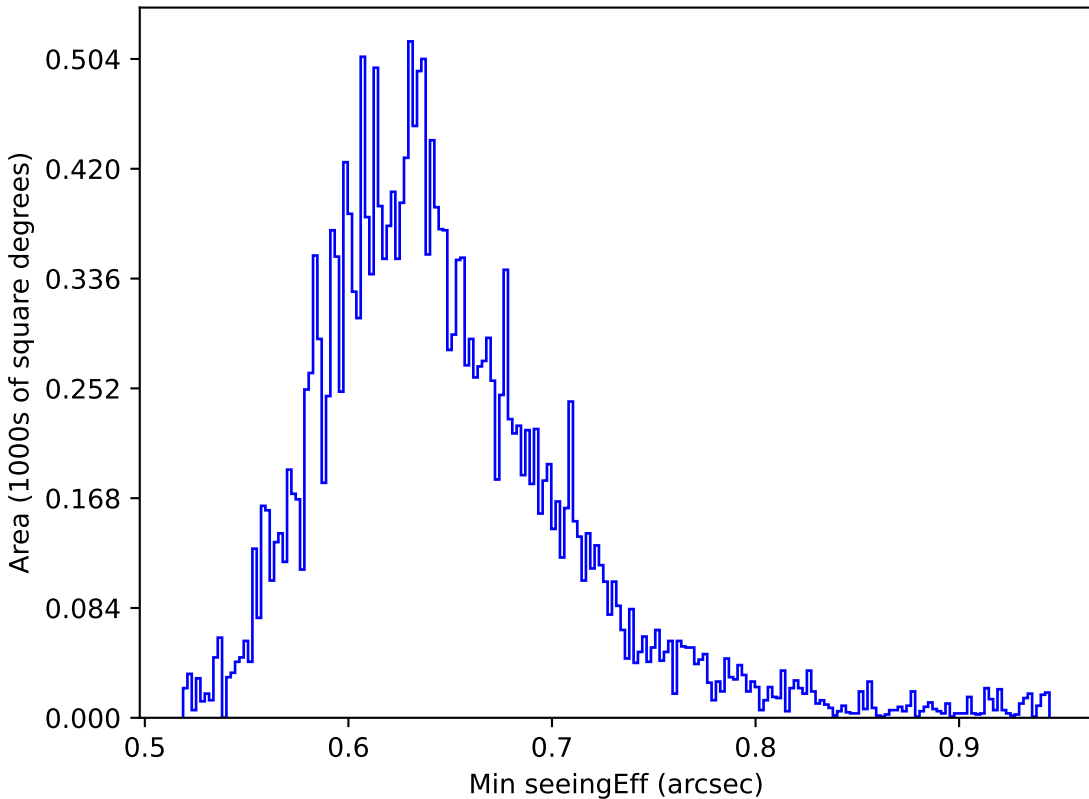
too_ignore_100_4v3.4_10yrs All sky y band: Min seeingEff
