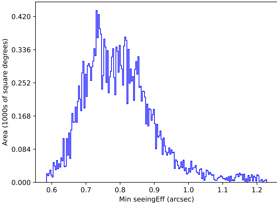
too_ignore_100_4v3.4_10yrs All sky u band: Min seeingEff
