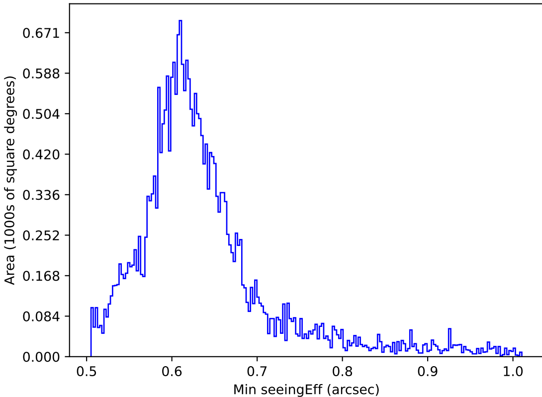
too_ignore_100_4v3.4_10yrs All sky i band: Min seeingEff
