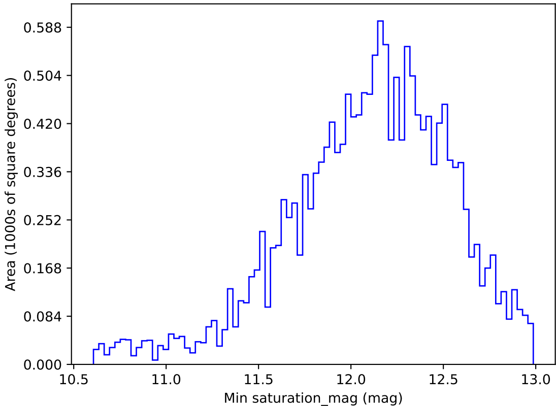
too_ignore_100_4v3.4_10yrs WFD z band: Min saturation_mag
