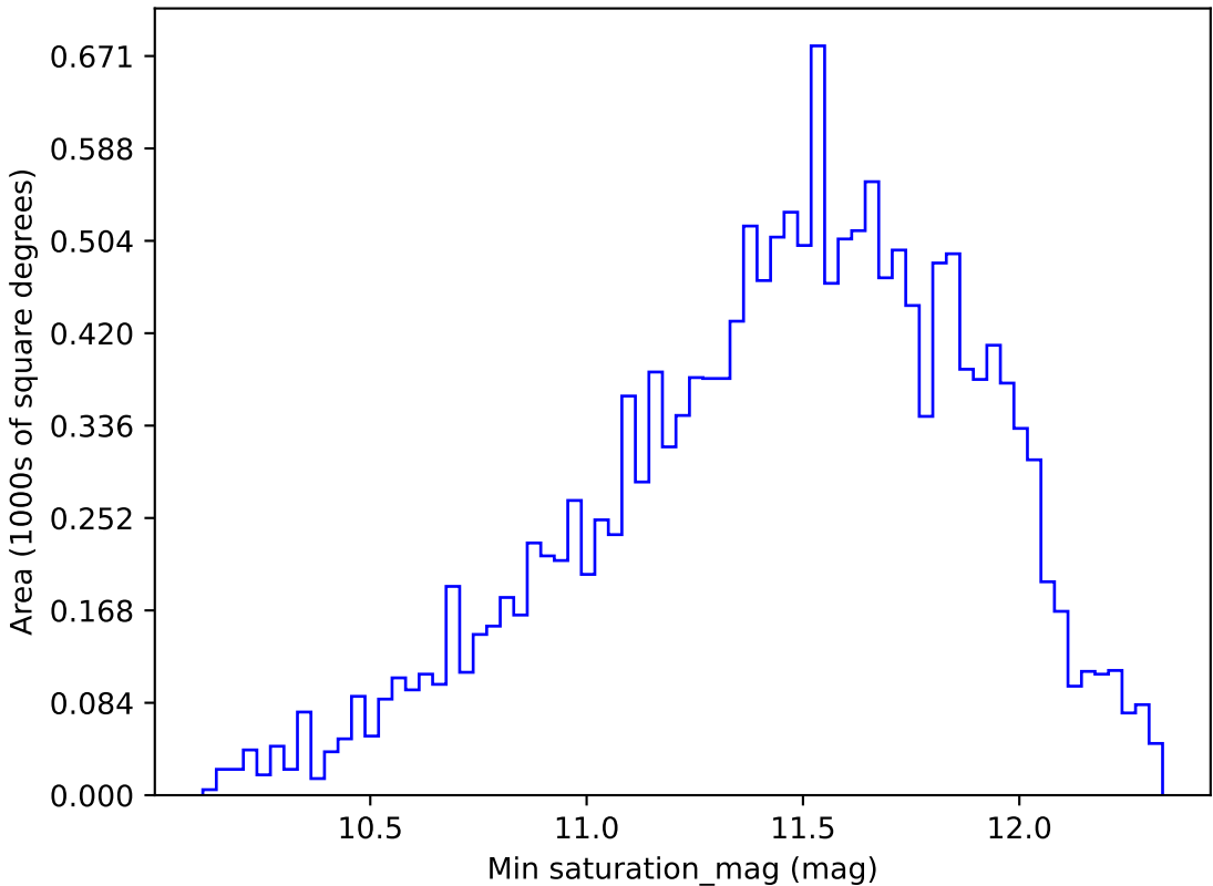
too_ignore_100_4v3.4_10yrs WFD u band: Min saturation_mag
