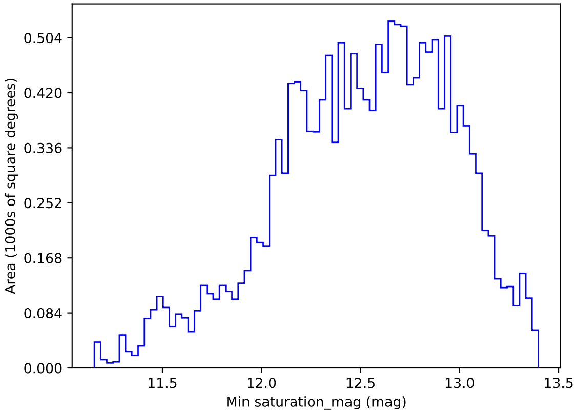
too_ignore_100_4v3.4_10yrs WFD r band: Min saturation_mag
