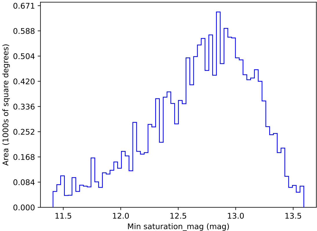
too_ignore_100_4v3.4_10yrs WFD g band: Min saturation_mag
