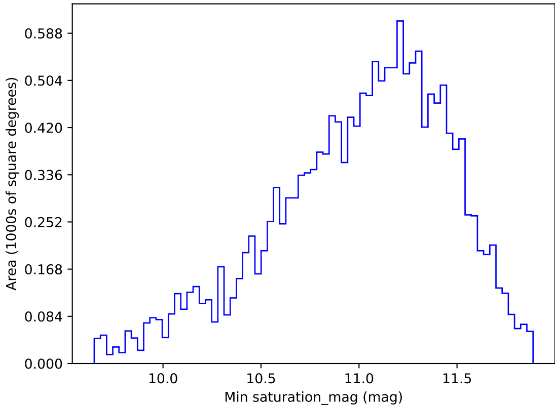
too_ignore_100_4v3.4_10yrs WFD all bands: Min saturation_mag
