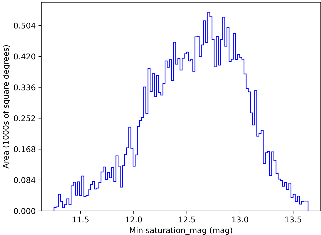
too_ignore_100_4v3.4_10yrs All sky r band: Min saturation_mag
