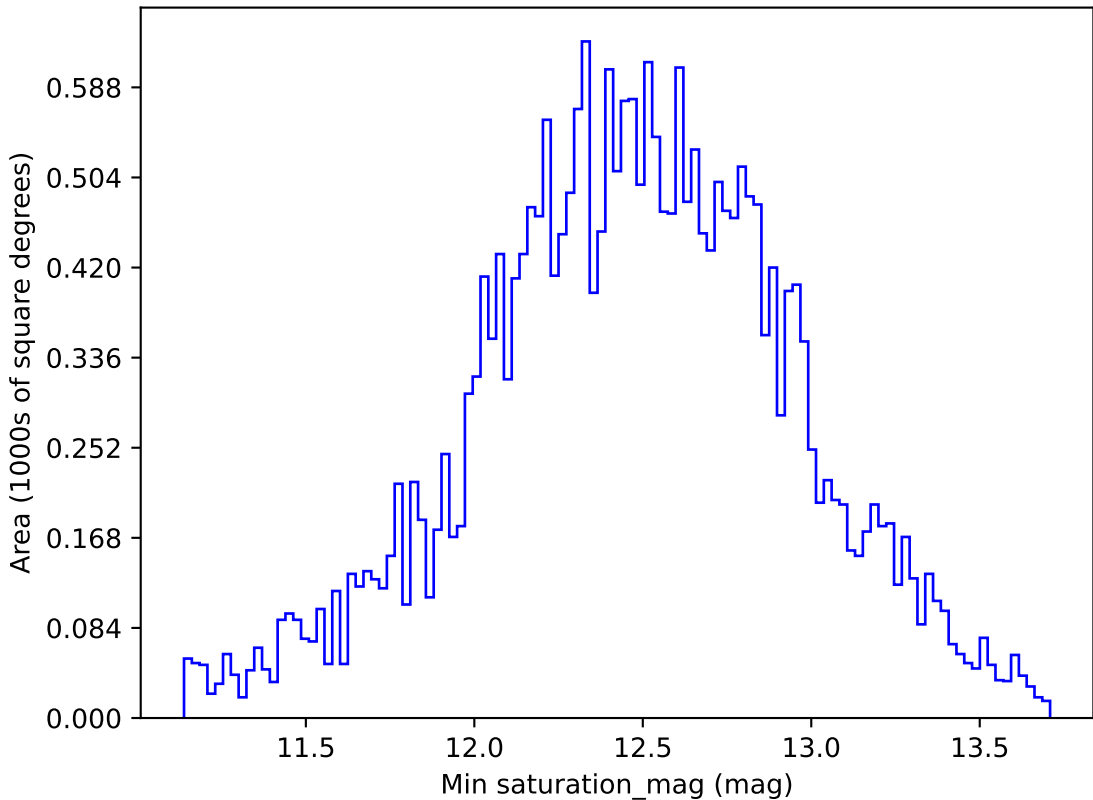
too_ignore_100_4v3.4_10yrs All sky i band: Min saturation_mag
