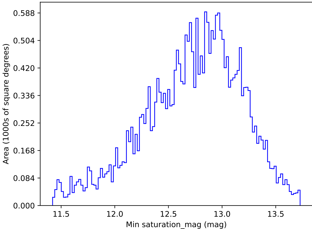
too_ignore_100_4v3.4_10yrs All sky g band: Min saturation_mag
