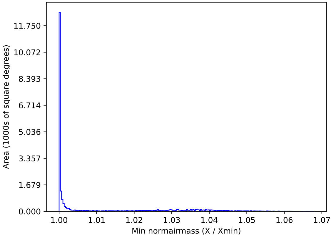
too_ignore_100_4v3.4_10yrs All sky u band: Min normairmass
