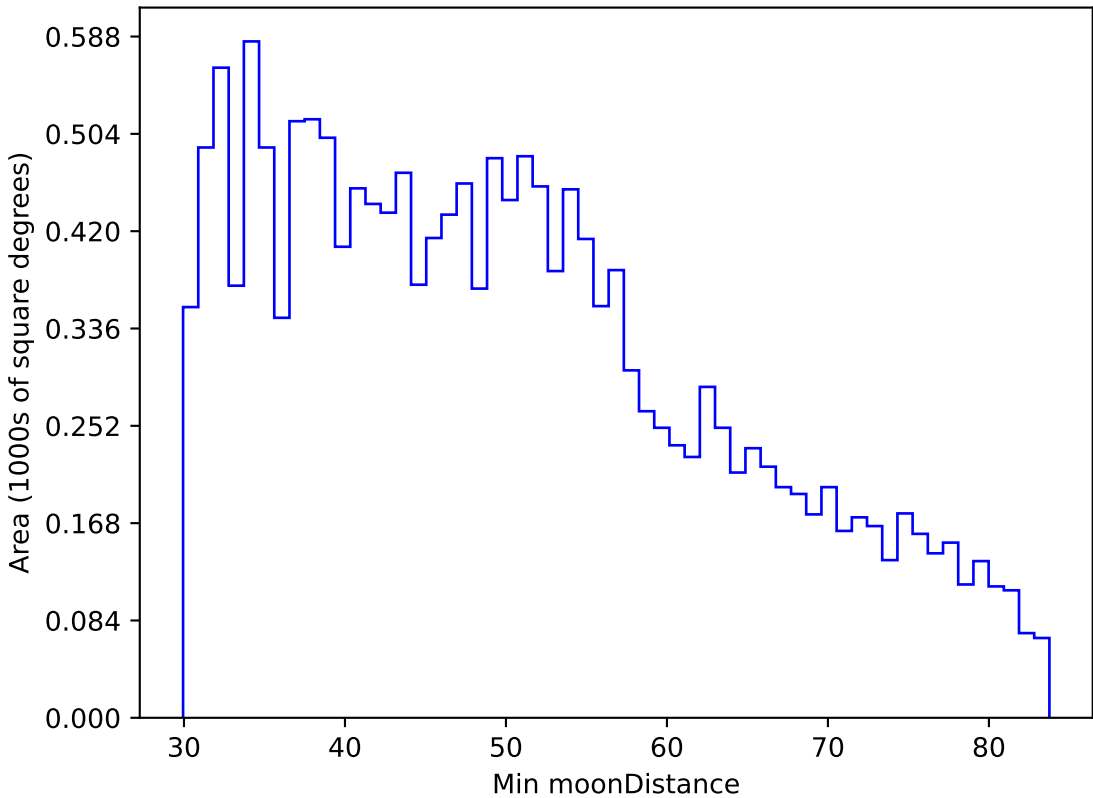
too_ignore_100_4v3.4_10yrs WFD u band: Min moonDistance
