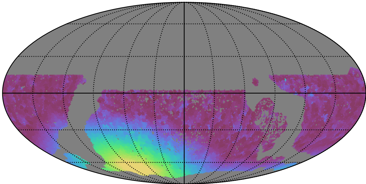
too_ignore_100_4v3.4_10yrs WFD r band: Min moonDistance
