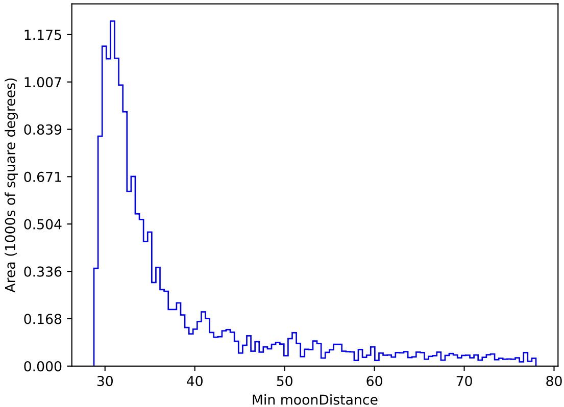
too_ignore_100_4v3.4_10yrs WFD r band: Min moonDistance
