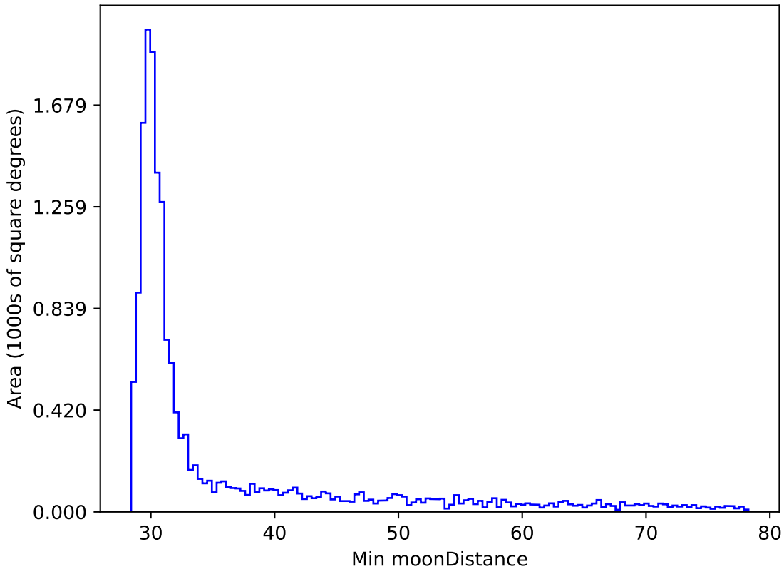
too_ignore_100_4v3.4_10yrs WFD i band: Min moonDistance
