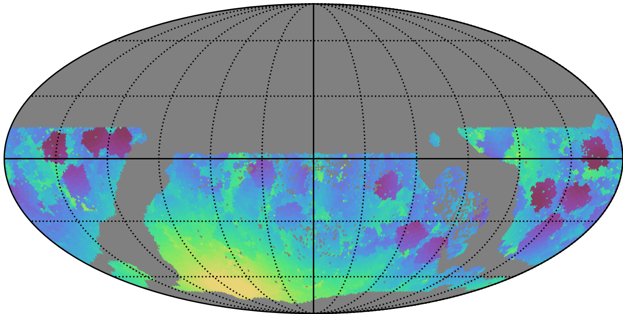
too_ignore_100_4v3.4_10yrs WFD g band: Min moonDistance
