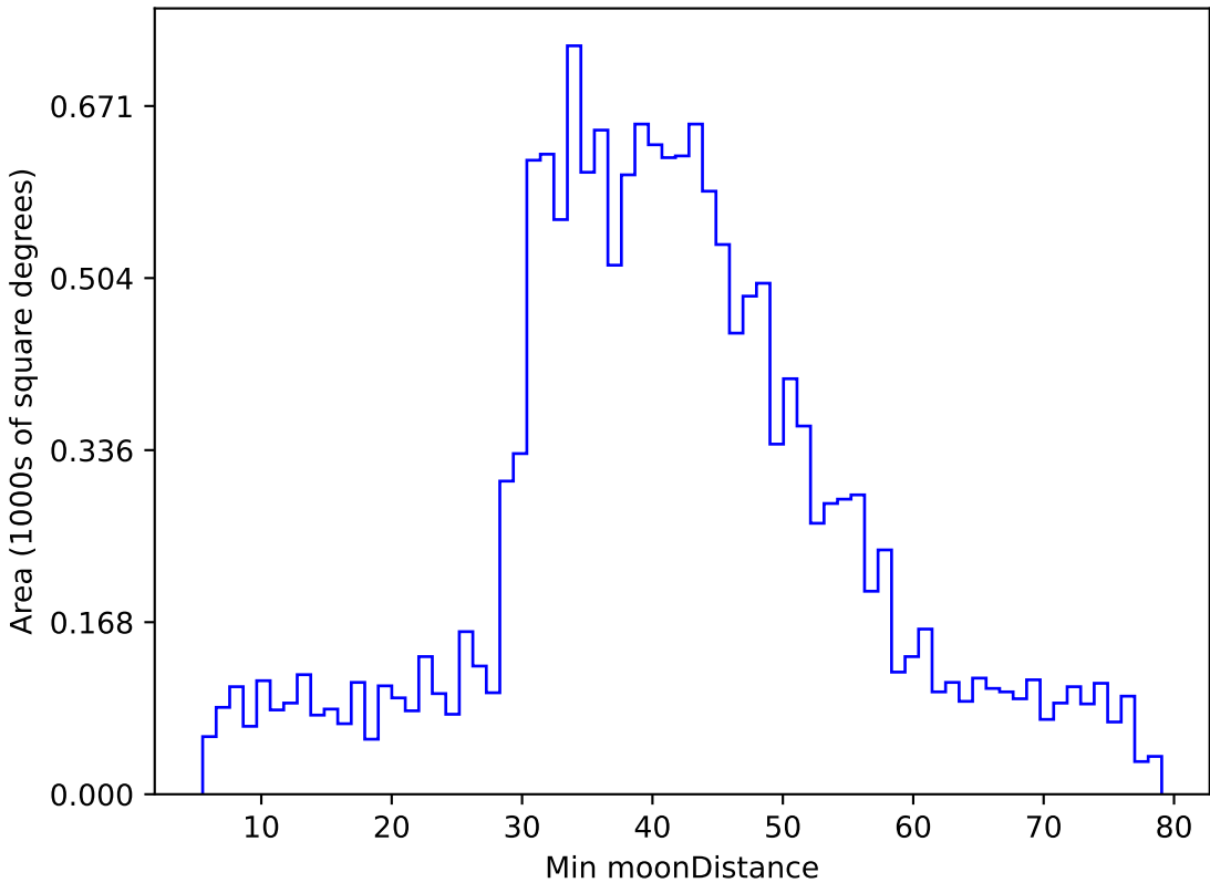
too_ignore_100_4v3.4_10yrs WFD g band: Min moonDistance
