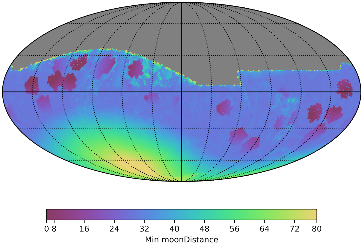
too_ignore_100_4v3.4_10yrs All sky z band: Min moonDistance
