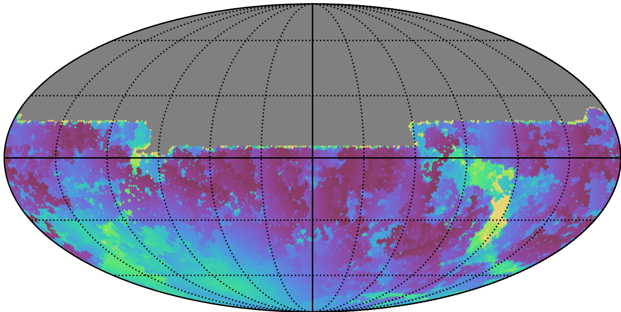
too_ignore_100_4v3.4_10yrs All sky u band: Min moonDistance
