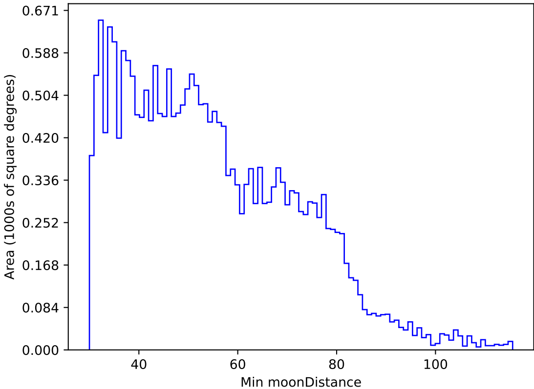
too_ignore_100_4v3.4_10yrs All sky u band: Min moonDistance
