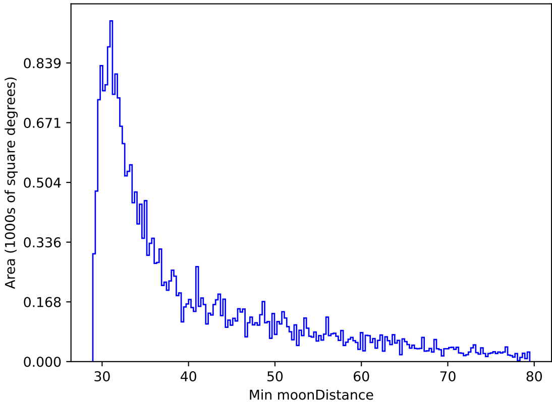
too_ignore_100_4v3.4_10yrs All sky r band: Min moonDistance
