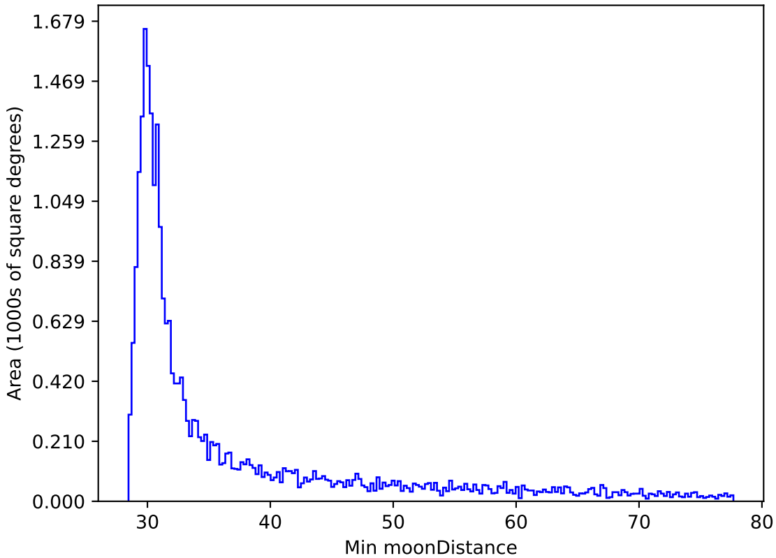
too_ignore_100_4v3.4_10yrs All sky i band: Min moonDistance
