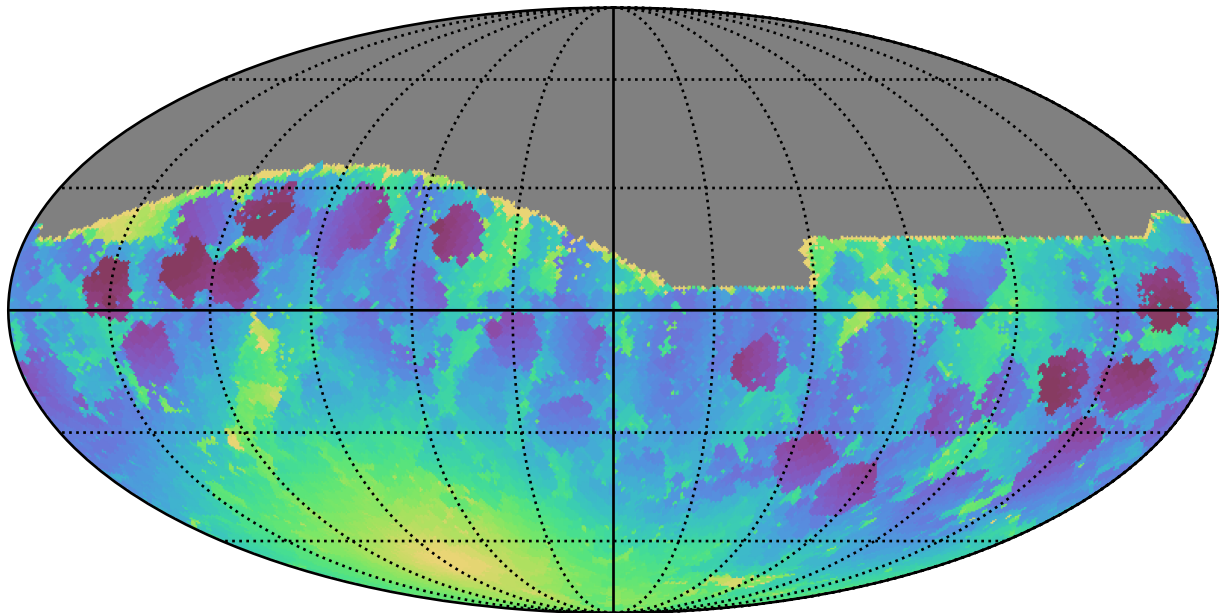
too_ignore_100_4v3.4_10yrs All sky g band: Min moonDistance
