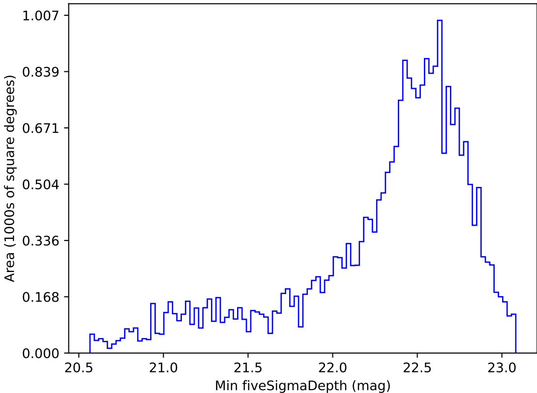
too_ignore_100_4v3.4_10yrs Yr 1 z band: Min fiveSigmaDepth
