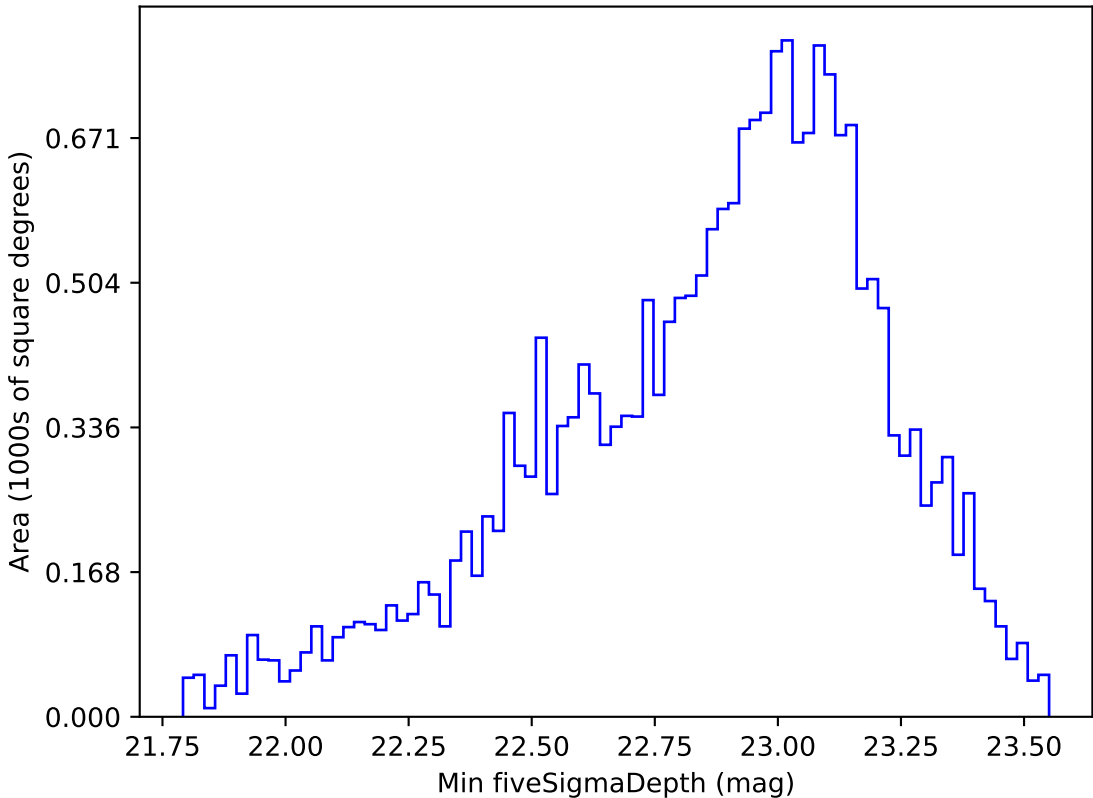
too_ignore_100_4v3.4_10yrs Yr 1 u band: Min fiveSigmaDepth
