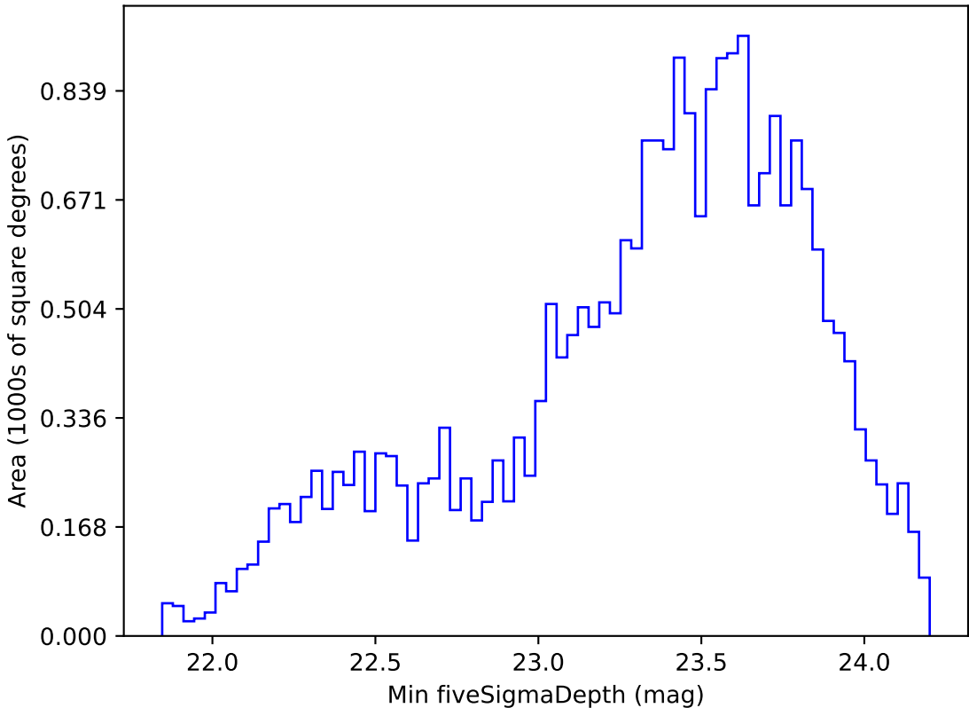
too_ignore_100_4v3.4_10yrs Yr 1 r band: Min fiveSigmaDepth
