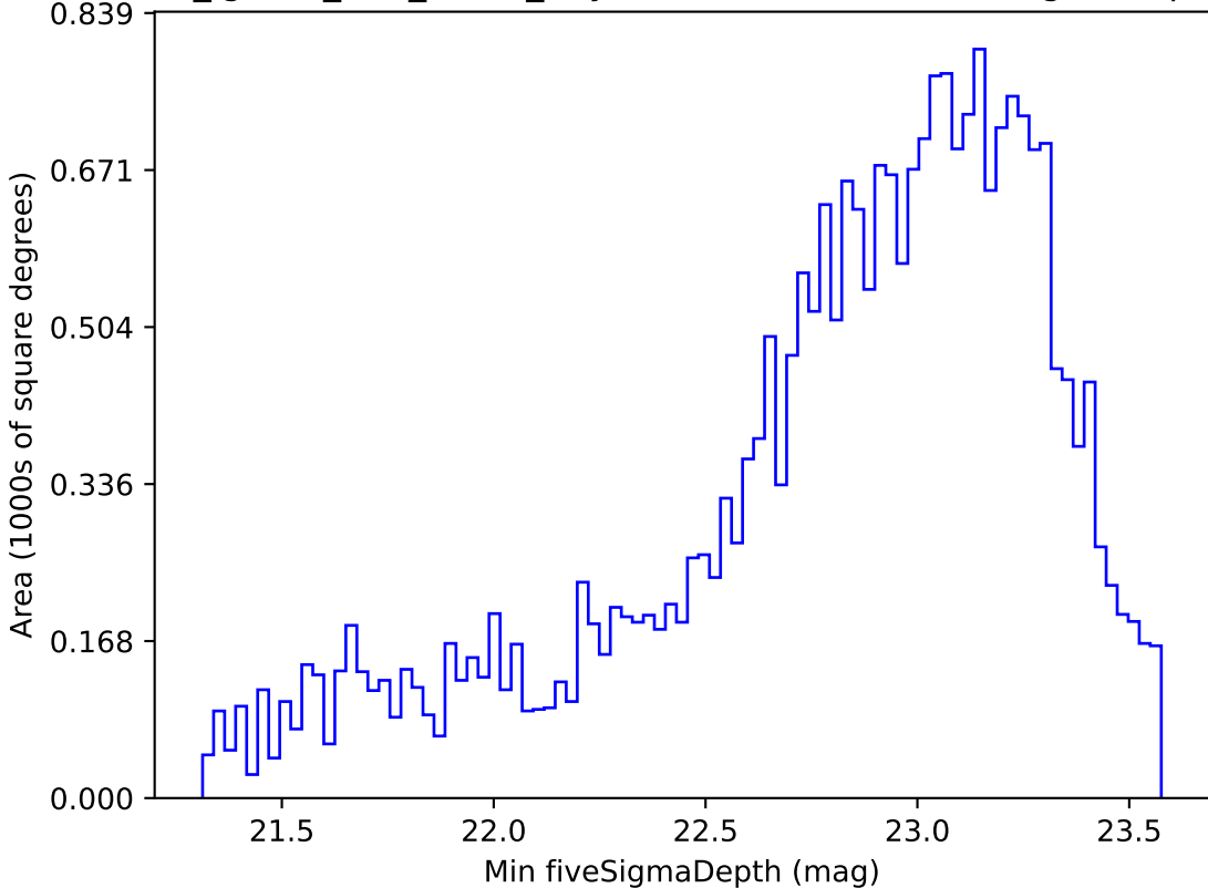
too_ignore_100_4v3.4_10yrs Yr 1 i band: Min fiveSigmaDepth
