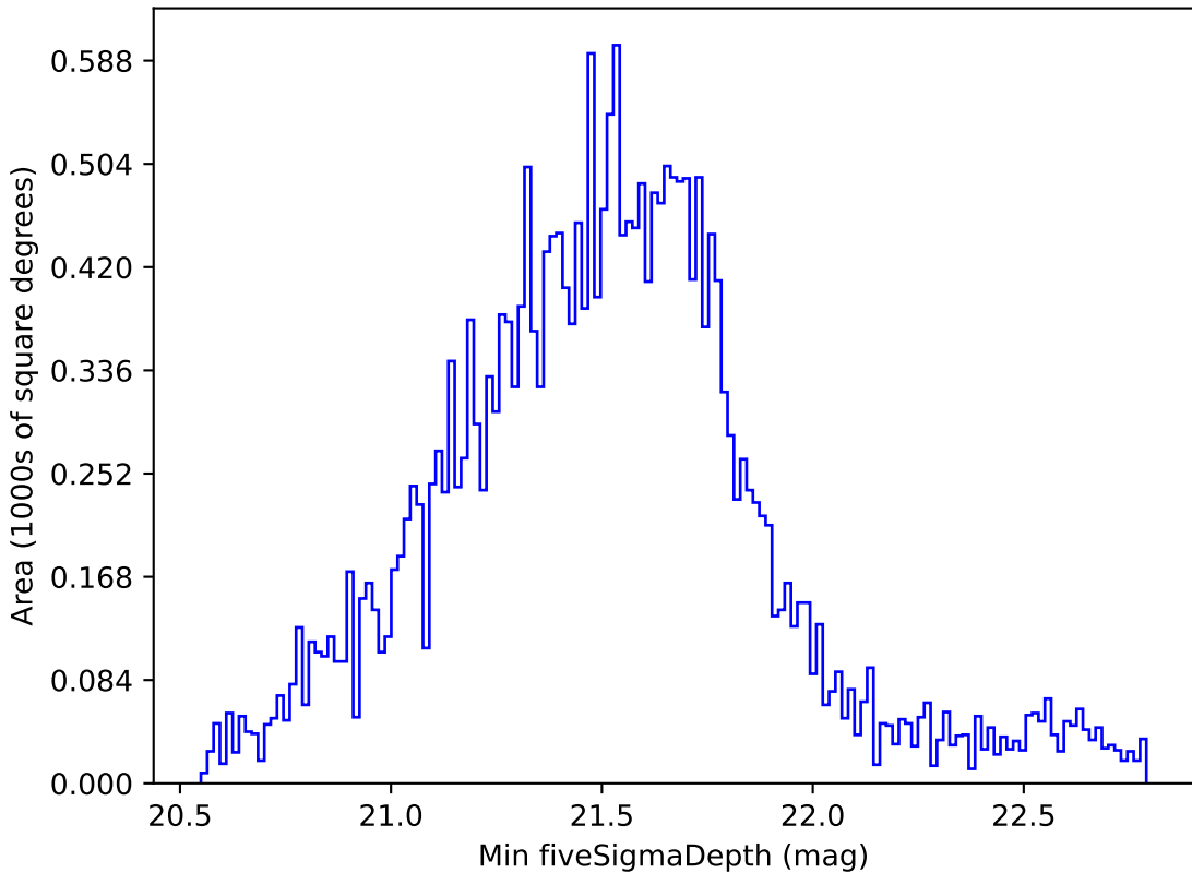
too_ignore_100_4v3.4_10yrs Yr 1 all bands: Min fiveSigmaDepth
