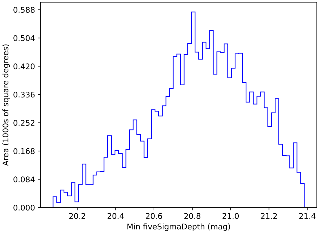
too_ignore_100_4v3.4_10yrs WFD y band: Min fiveSigmaDepth
