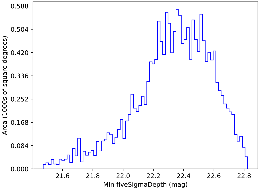
too_ignore_100_4v3.4_10yrs WFD u band: Min fiveSigmaDepth
