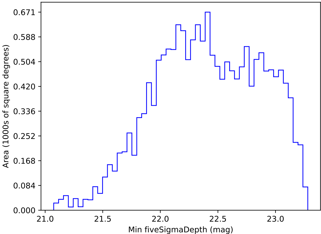
too_ignore_100_4v3.4_10yrs WFD r band: Min fiveSigmaDepth
