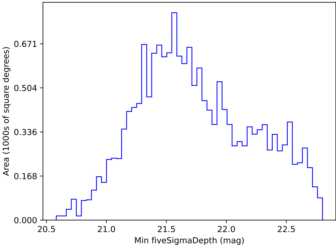
too_ignore_100_4v3.4_10yrs WFD i band: Min fiveSigmaDepth
