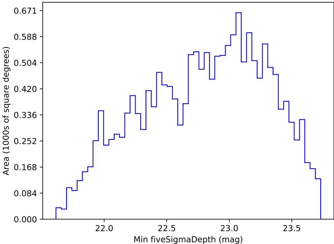
too_ignore_100_4v3.4_10yrs WFD g band: Min fiveSigmaDepth
