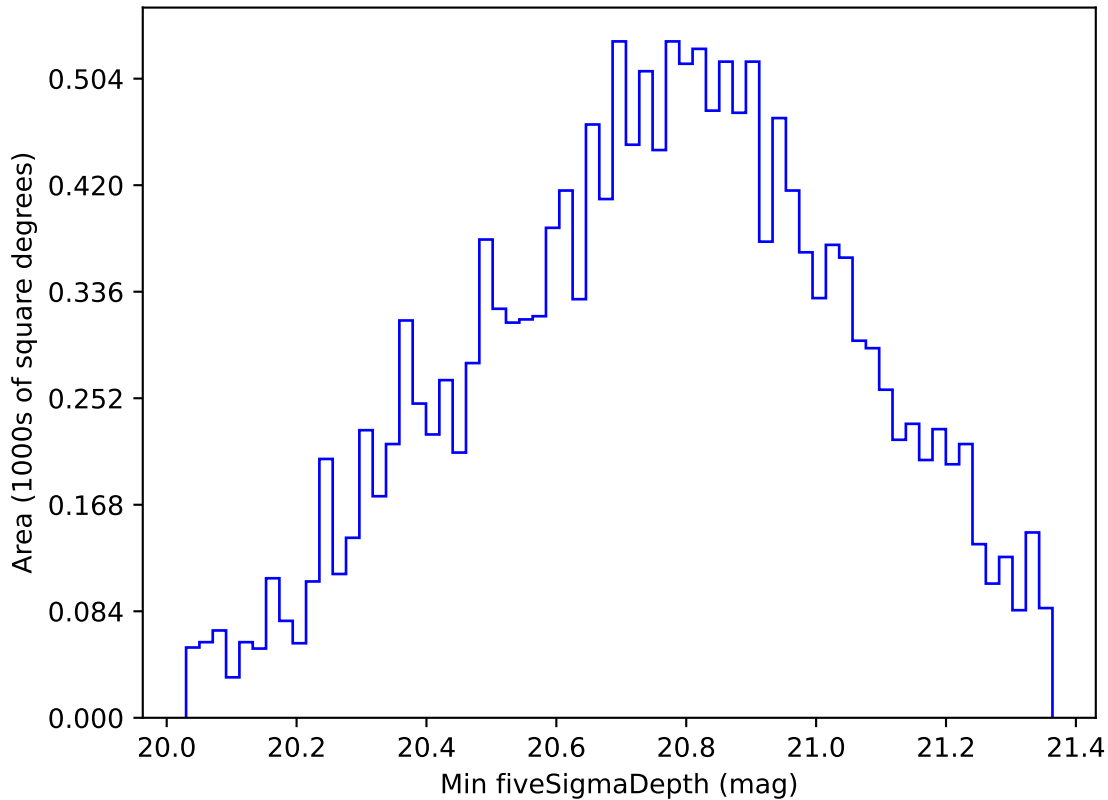
too_ignore_100_4v3.4_10yrs WFD all bands: Min fiveSigmaDepth
