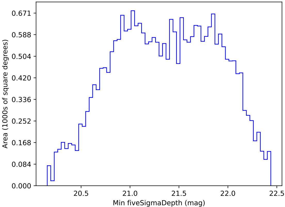
too_ignore_100_4v3.4_10yrs All sky z band: Min fiveSigmaDepth
