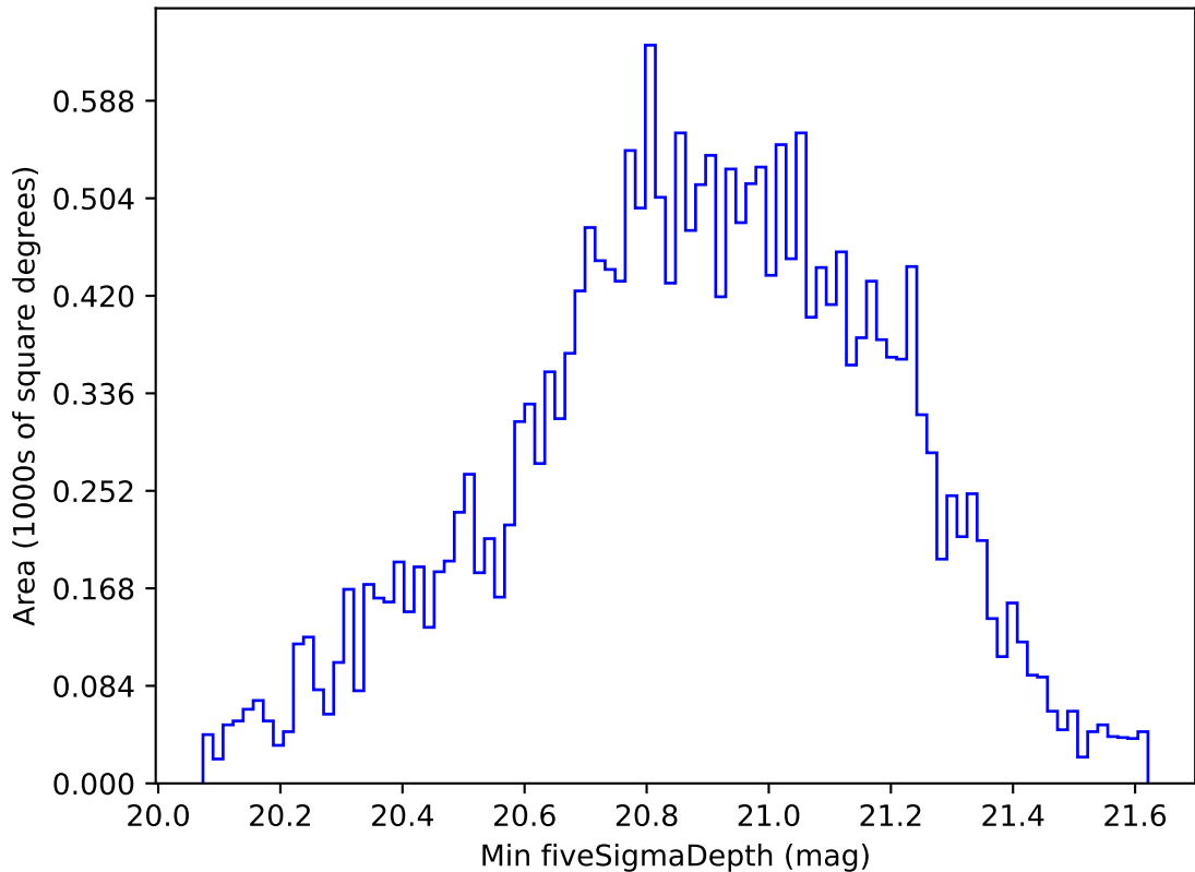
too_ignore_100_4v3.4_10yrs All sky y band: Min fiveSigmaDepth
