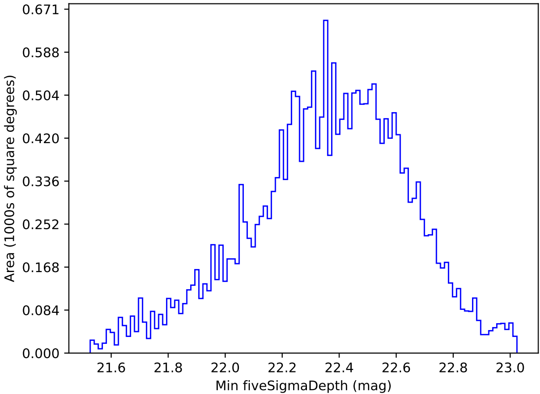
too_ignore_100_4v3.4_10yrs All sky u band: Min fiveSigmaDepth
