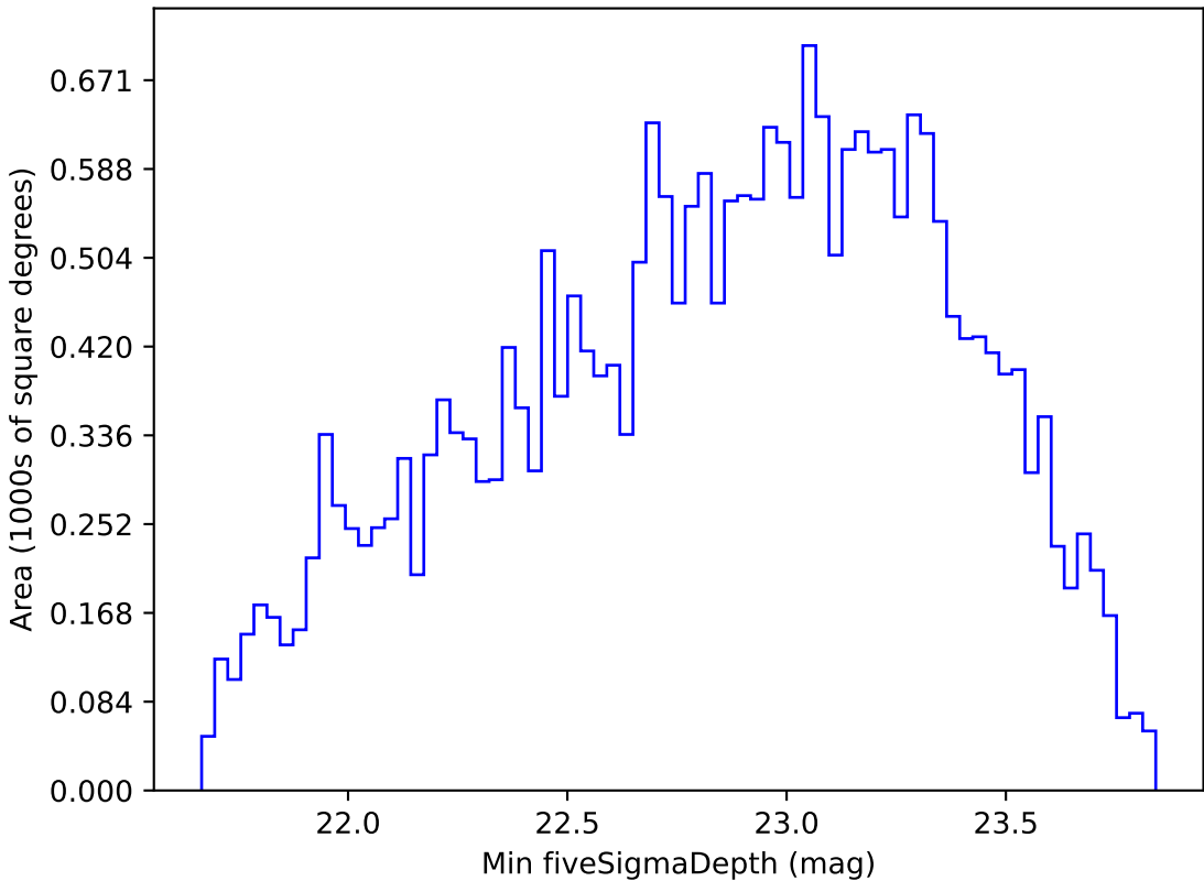
too_ignore_100_4v3.4_10yrs All sky g band: Min fiveSigmaDepth
