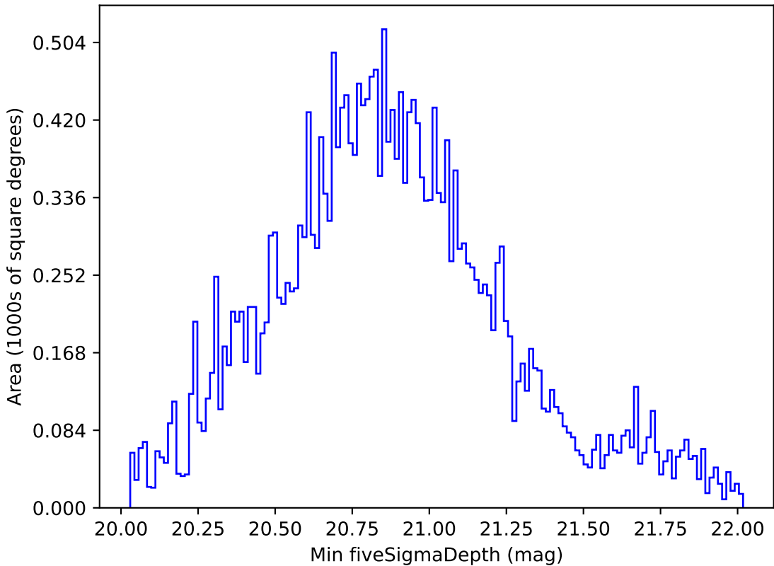
too_ignore_100_4v3.4_10yrs All sky all bands: Min fiveSigmaDepth
