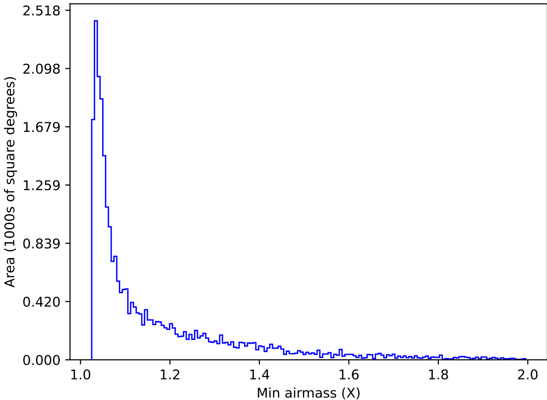
too_ignore_100_4v3.4_10yrs Yr 1 z band: Min airmass
