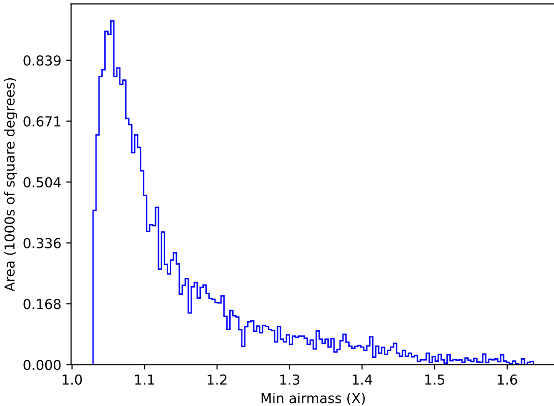
too_ignore_100_4v3.4_10yrs Yr 1 u band: Min airmass
