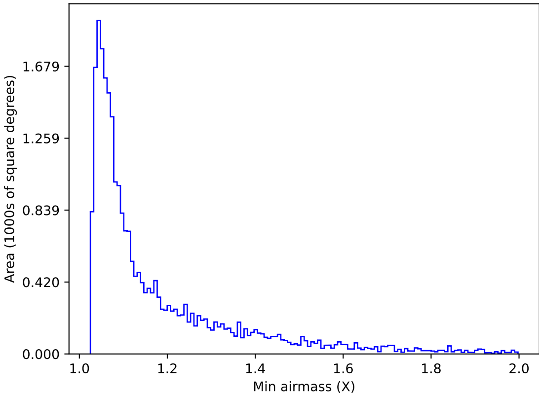
too_ignore_100_4v3.4_10yrs Yr 1 g band: Min airmass
