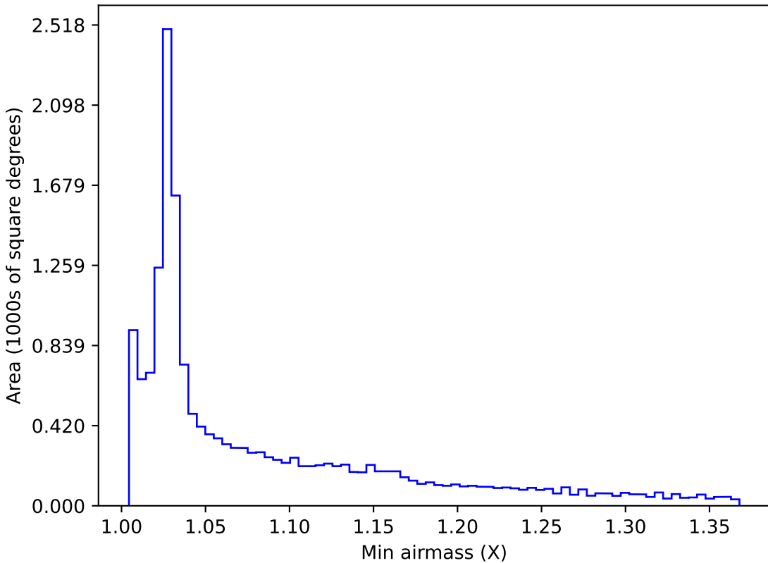
too_ignore_100_4v3.4_10yrs WFD z band: Min airmass
