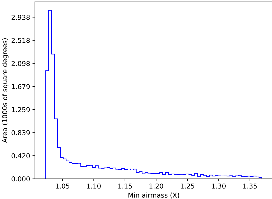
too_ignore_100_4v3.4_10yrs WFD y band: Min airmass
