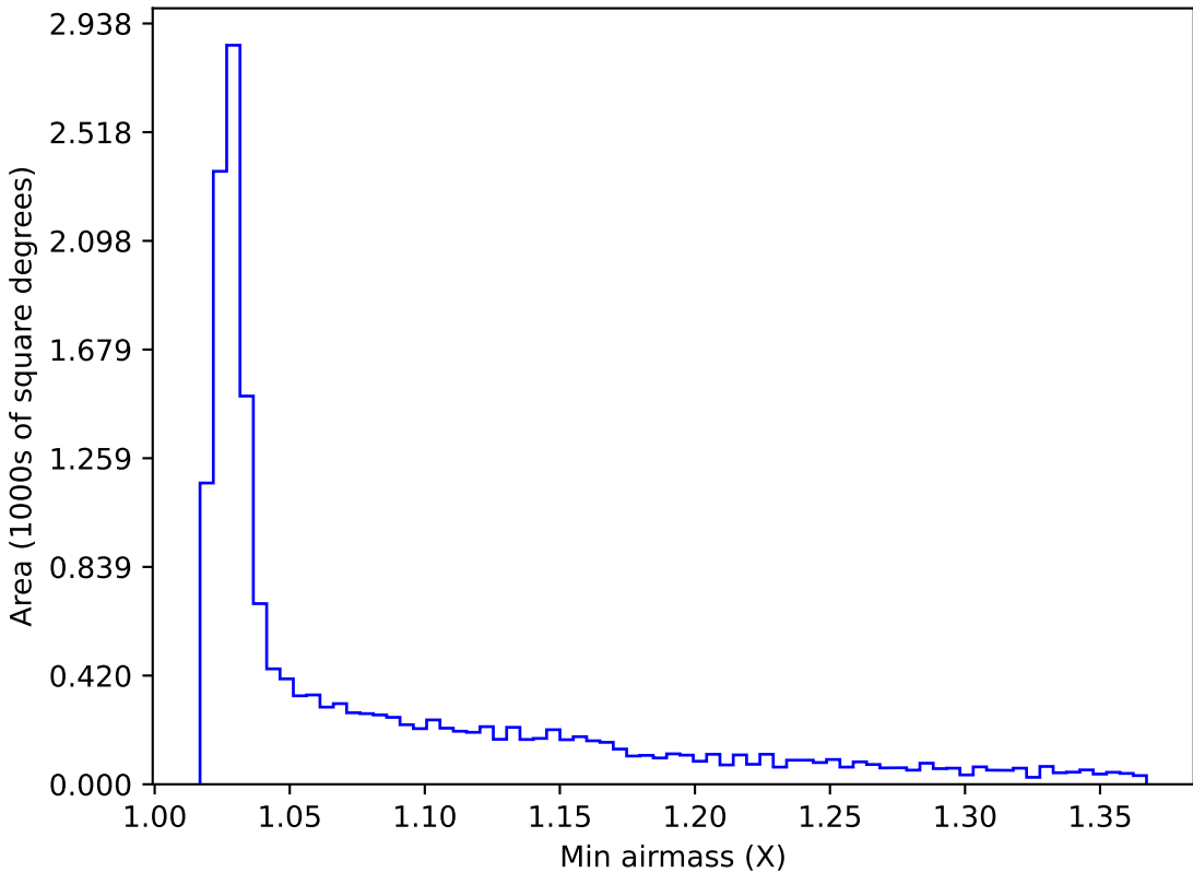
too_ignore_100_4v3.4_10yrs WFD r band: Min airmass
