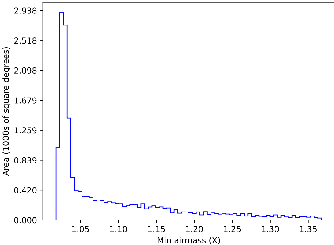
too_ignore_100_4v3.4_10yrs WFD i band: Min airmass
