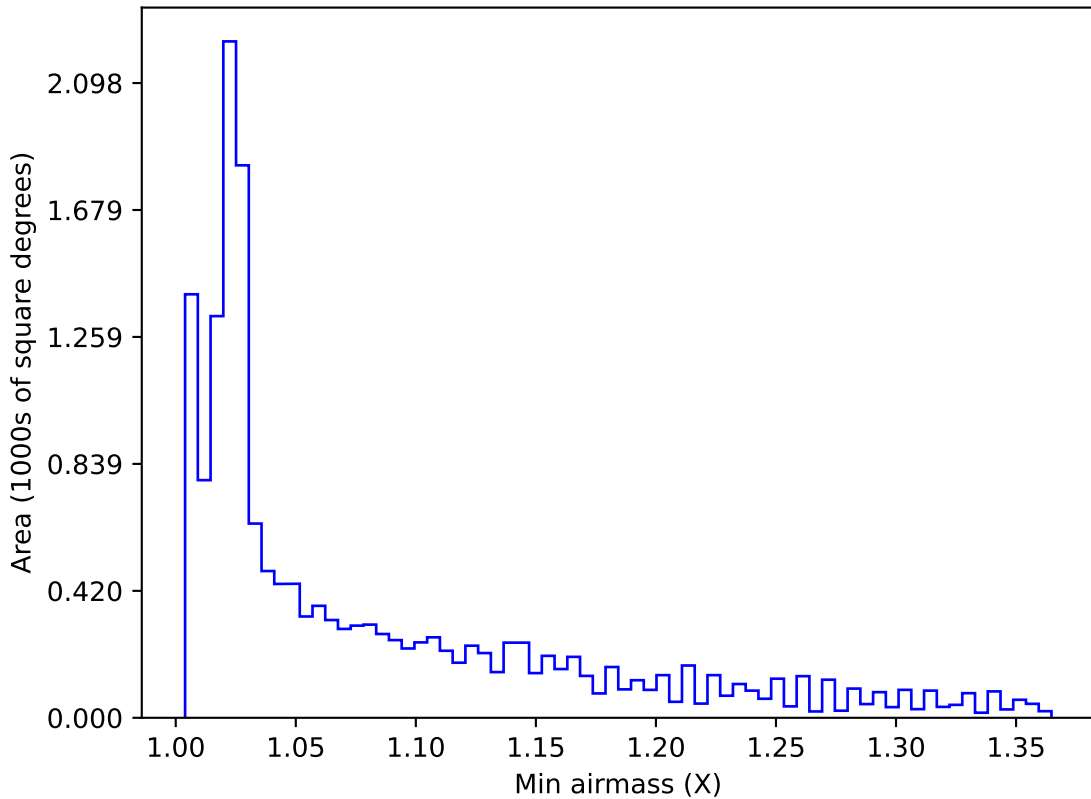
too_ignore_100_4v3.4_10yrs WFD all bands: Min airmass
