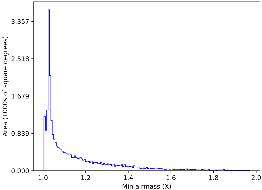
too_ignore_100_4v3.4_10yrs All sky z band: Min airmass
