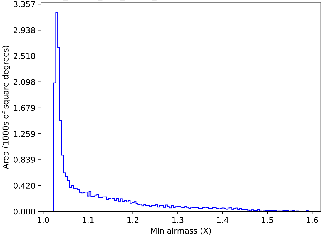
too_ignore_100_4v3.4_10yrs All sky y band: Min airmass
